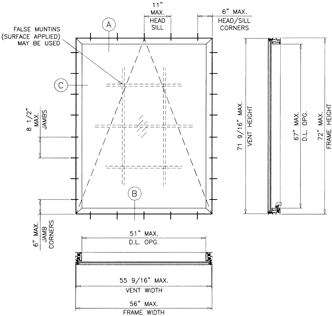
TYPICAL ELEVATION
